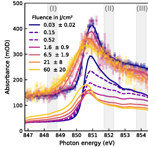
FIG. 3. Fluence-dependent NiL 3 -edge spectra, measured (top) and simulated (bottom). The fluence of events contributing to each spectrum is given in the legend in terms of mean and standard deviation. Dashed simulated spectra do not have a corresponding measurement. The regions of interest from which absorbance changes shown in panels b), d), and e) of Fig. 4 were quantified are shaded and labeled (I), (II), and (III), respectively. The error bars are shown for the measured spectra and represent the 95% confidence intervals for each bin of 102 meV width; solid lines of the measured spectra are smoothed using a Savitzky-Golay filter using windows of 21 bins and 4th-order polynomials. The experimental spectra are vertically offset by 100 mOD.
