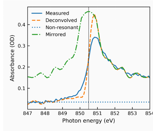
FIG. 9. Derivation of absorption lengths as input parameters , reconstructed from a measured ground-state spectrum (blue line). The non-resonant absorption level (blue dots) was determined from the pre-edge region. The measured resonant absorption length was deconvolved with the experimental resolution (orange dashes) and mirrored around the rising edge to retrieve a symmetric resonant absorption length around the resonance (green dot-dashed line). See main text for details.
